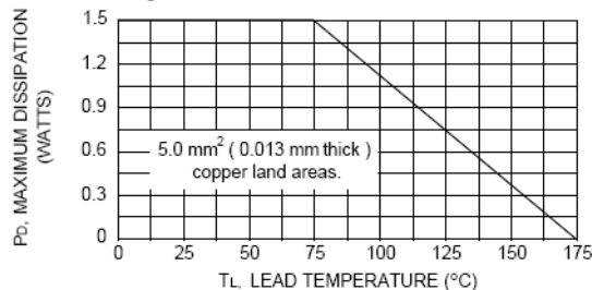
Fig. 1 POWER TEMPERATURE DERATING CURVE
